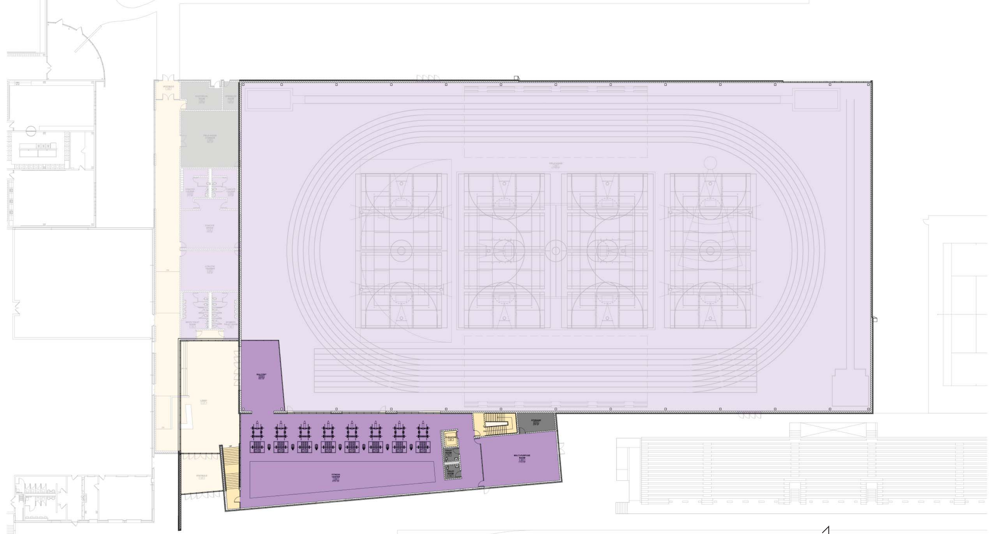
PROPOSED SECOND FLOOR PLAN
